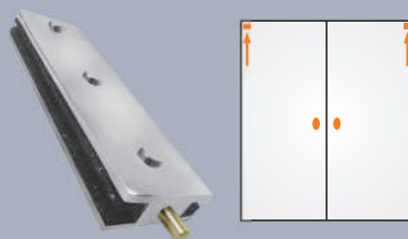
1101 Jumbo | Dobradiça superior especial Jumbo | Bisagra superior especial
