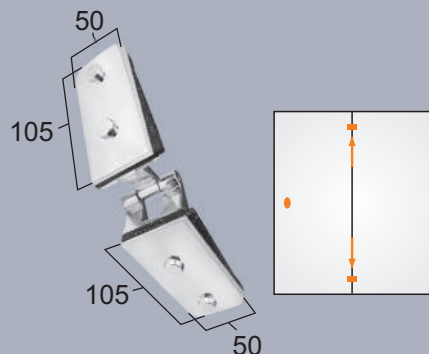
1117 Dobradiça horizontal dupla Bisagra horizontal doble
